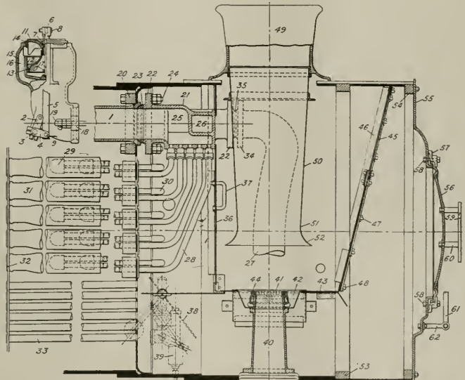
DETAILS OF SMOKEBOX, SUPERHEATER AND THROTTLE VALVE
